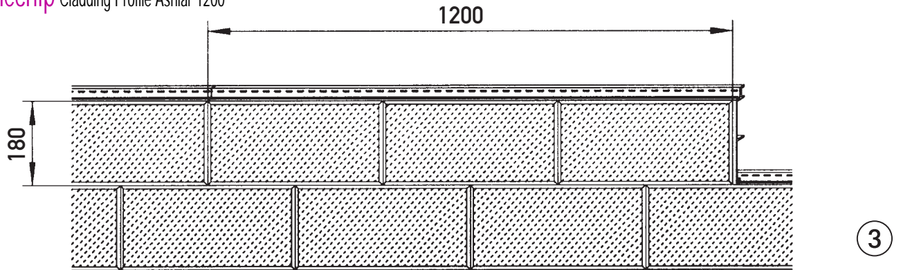
Cadre Stonechip Cladding Profile Ashlar 1200
