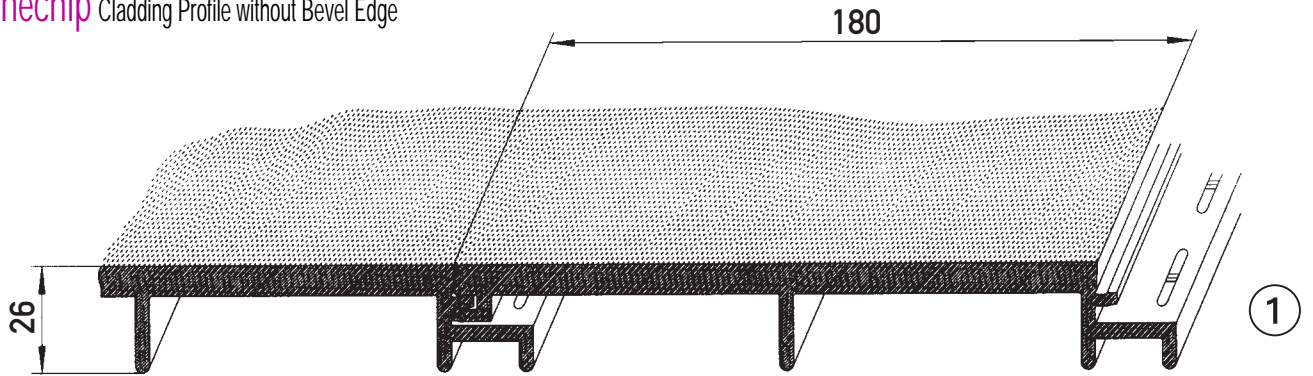
Cadre Stonechip Cladding Profile with Bevel Edge
